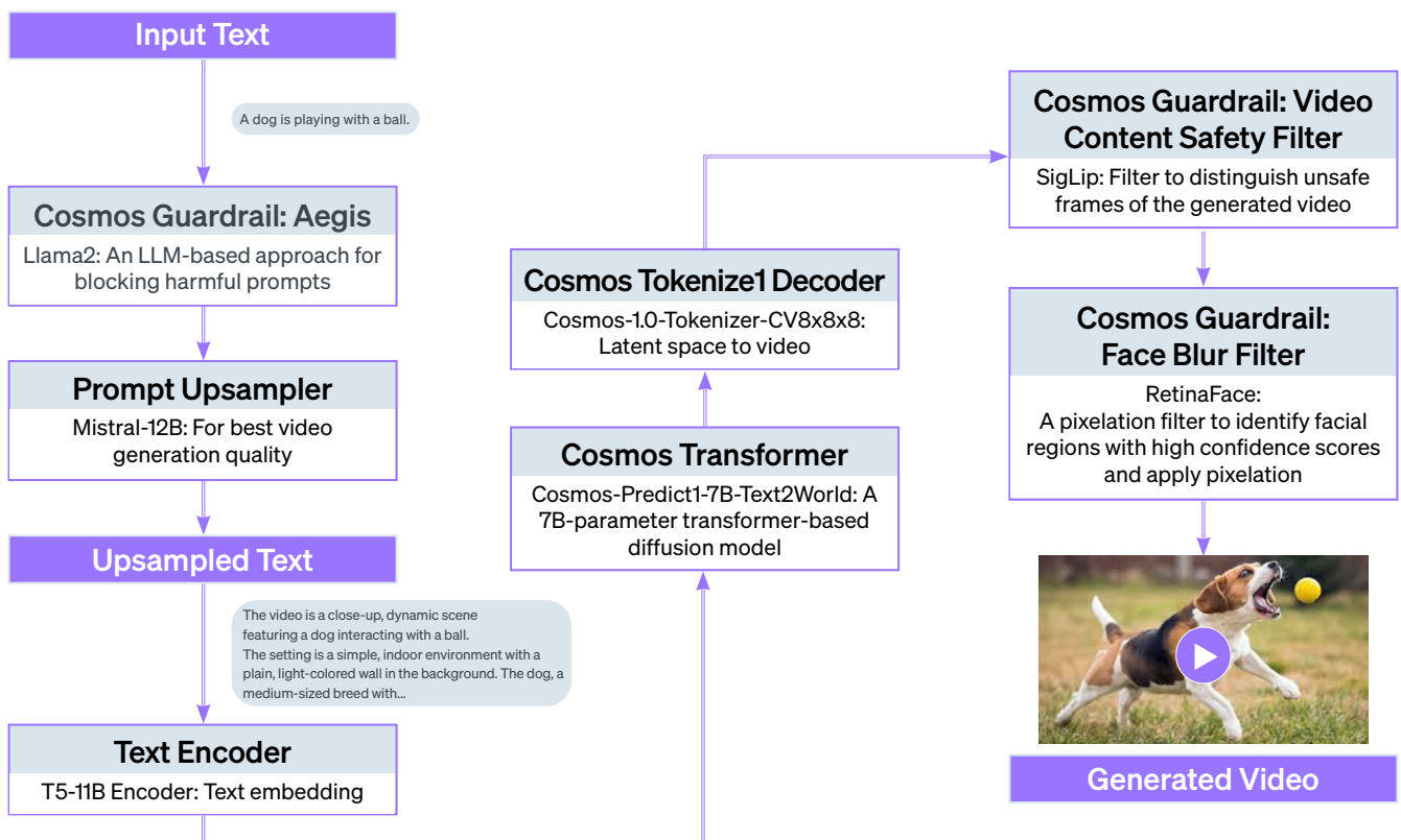
[Figure 1. Cosmos-Predict1-7B + Cosmos Guardrail diagram]
